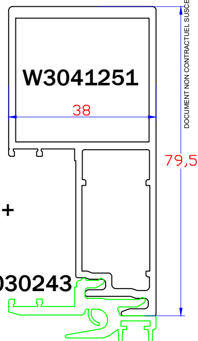
Montant Central forte inertie
